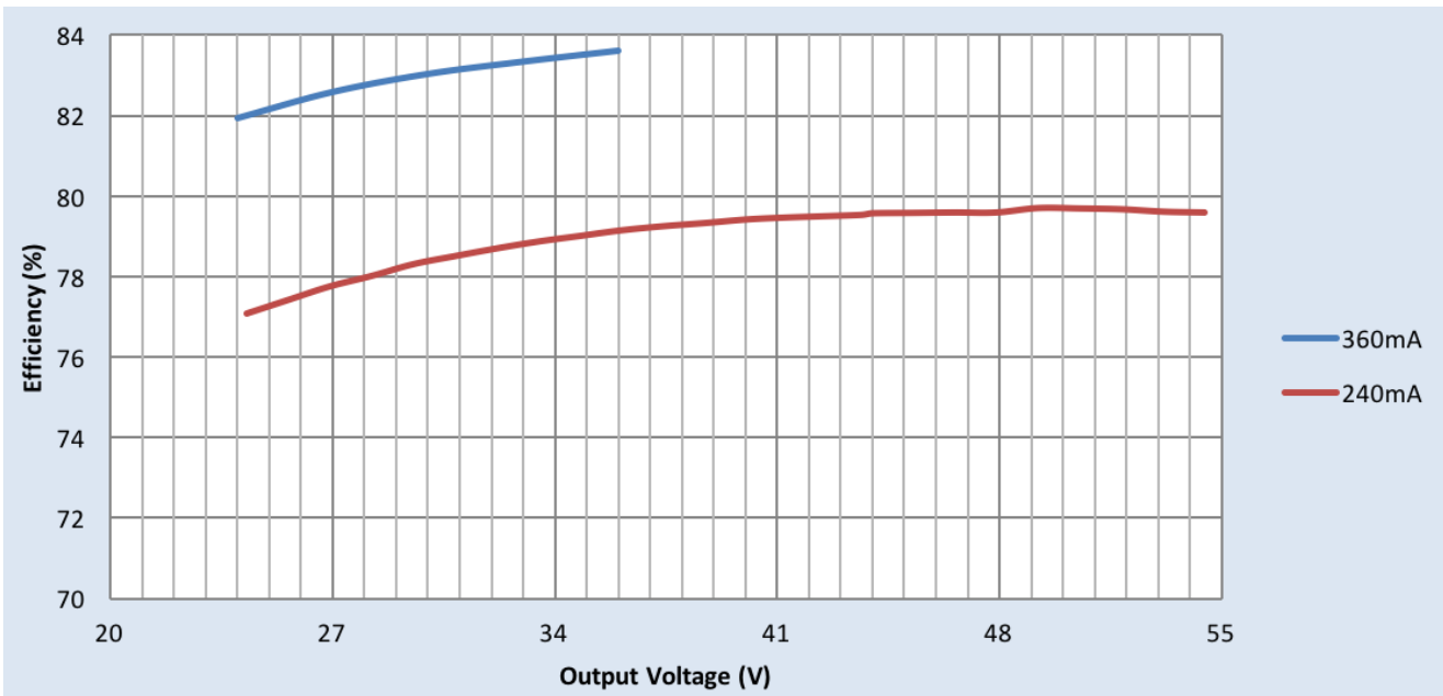
Efficiency Vs. Output Voltage at 120Vac
