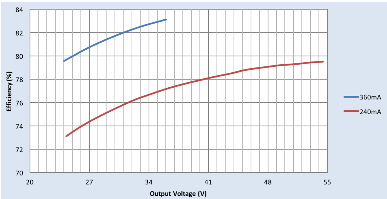
Efficiency Vs. Output Voltage at 277Vac
